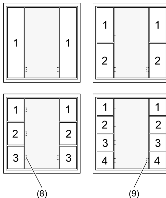
Figure 2: Channel assignment of wall transmitter module 1-gang, 2-gang, 3-gang and 4-gang
