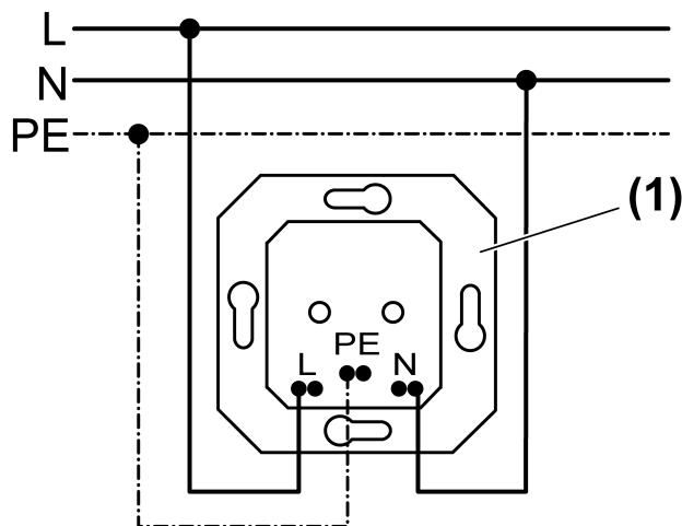
Figure 2: Connection diagram for single socket outlet
