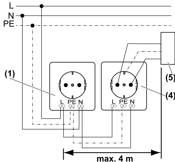
Figure 3: Connection diagram for socket outlet combination
